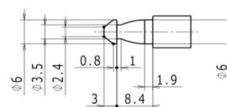
STRIKER SHAPE FOR REFERENCE
