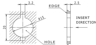
FITTING HOLE SHAPE (REFERENCE)
